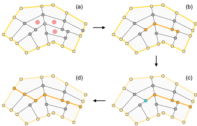
Figure 8: Generating streets to ensure reachability of newly generated parcels: (a) identify and group unreachable parcels (high-lighted with a red dot); (b) compute an L-shaped street access (in orange) for the group of unreachable parcels; (c) connect the L-shaped street access with the existing street network (in yellow) using a weighted shortest path (in orange) in the parcel corner graph, resulting in a street end (in cyan); and (d) connect the street end with the current street network to avoid generating a cul-de-sac.
